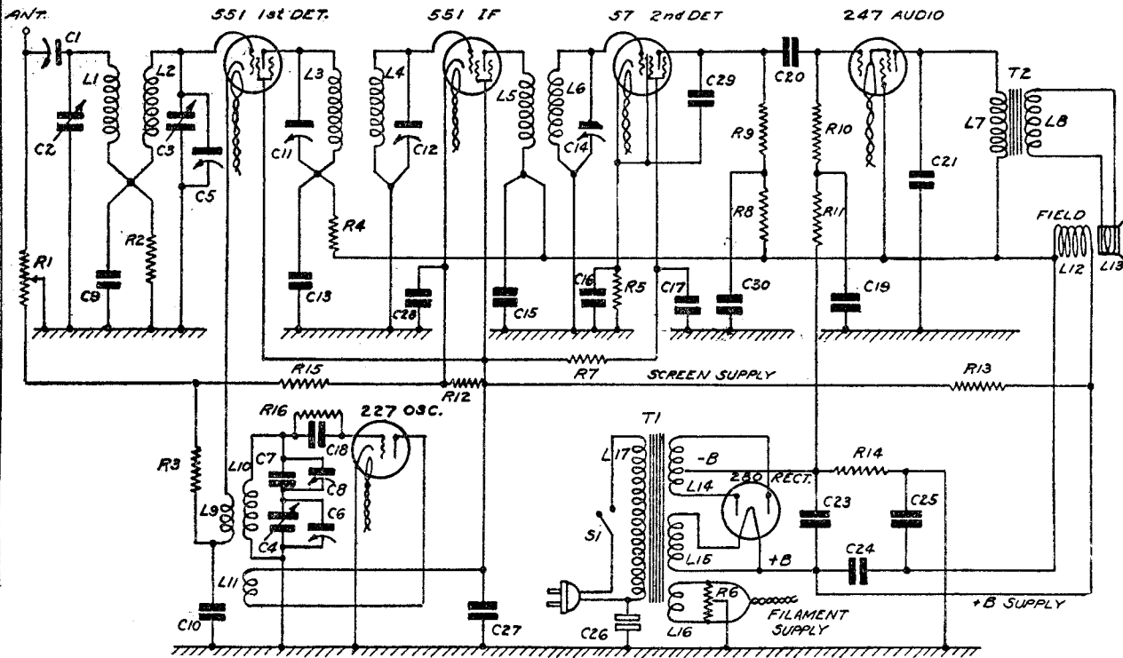
Schematic Diagram of Model 236 Receiver
